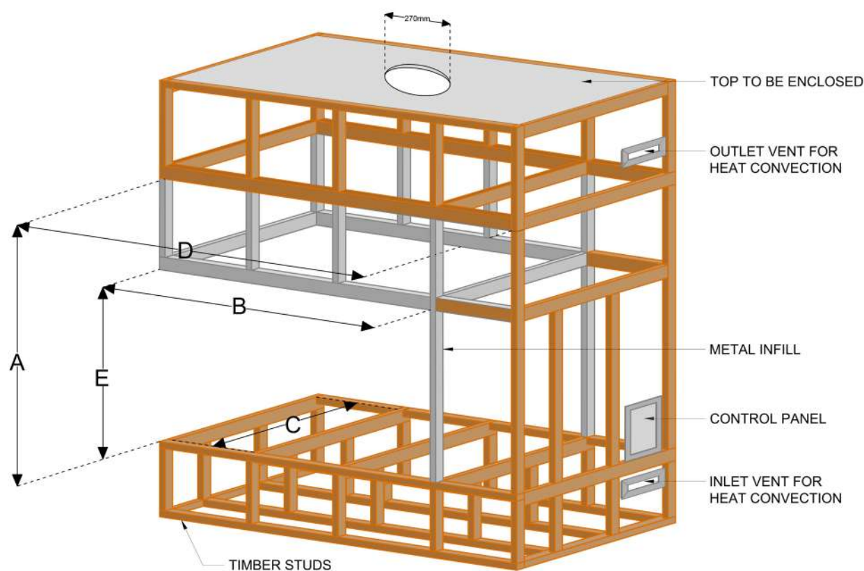
Figure 1.8 (Timber framing)
